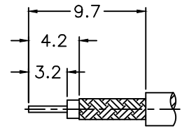
RECOMMENDED CABLE STRIPPING DIM'S (建議剝線尺寸)
