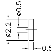
RECOMMENDED CABLE STRIPPING DIM'S (建議剝線尺寸)
